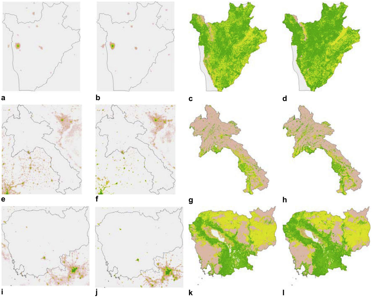
Figure 3. DMSP-OLS night-time light and MODIS land cover for three different countries with a high dependence on agriculture for the year 2001 and 2009. Nighttime light for Burundi 2001 and 2009. (a and b) and MODIS land cover for matching year (c and d). Lao People's Democratic Republic (e–h). Cambodia (i–l).
